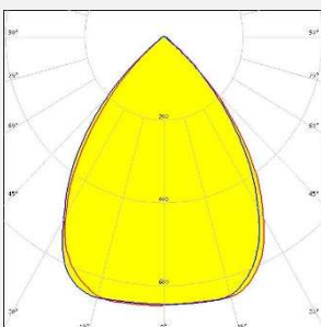
Beam Angle 60°
