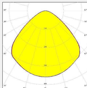
Beam Angle 110°
