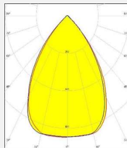
Beam Angle 60°
