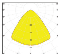
BEAM ANGLE 90°
