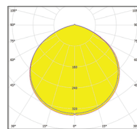
BEAM ANGLE 120°
