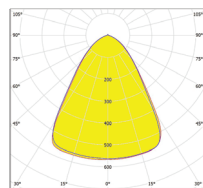
BEAM ANGLE 60°
