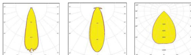
BEAM ANGLE 20° SPOT BEAM ANGLE 30° BEAM ANGLE 60°
