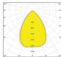
BEAM ANGLE 60°
