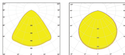
BEAM ANGLE 90° BEAM ANGLE 120°
